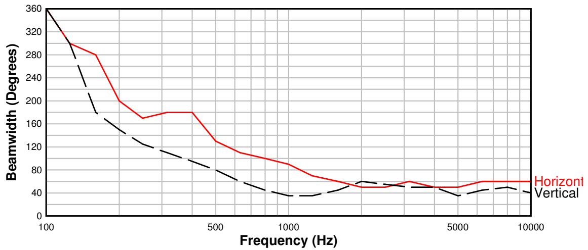
Beamwidth versus Frequency 212IM 60 x 40
