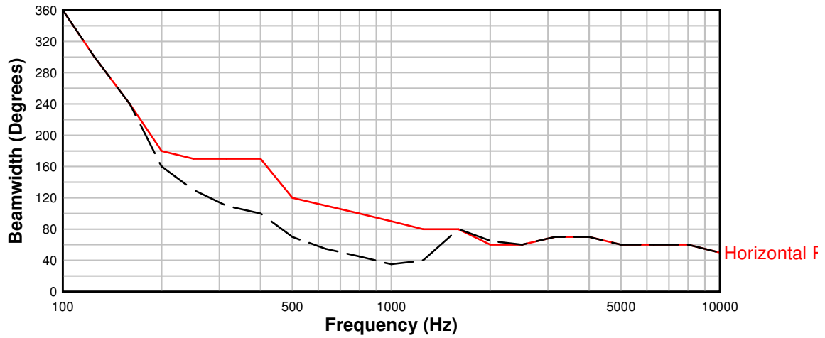
Beamwidth versus Frequency 212CIM Active
