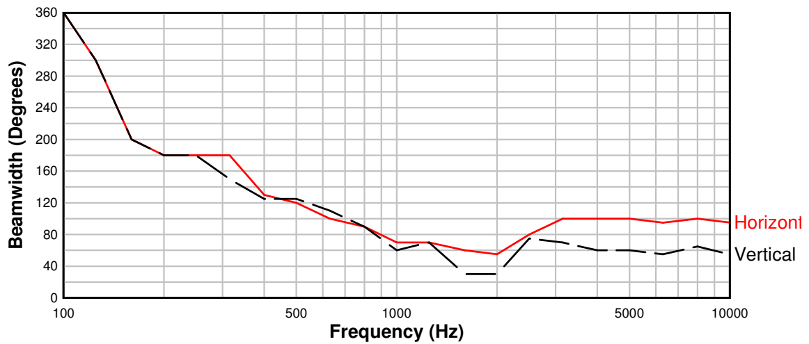
Beamwidth versus Frequency 115TW 105 X 60
