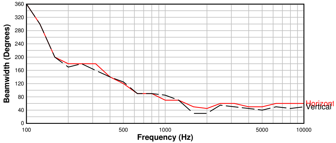
Beamwidth versus Frequency 115RW 60 X 40
