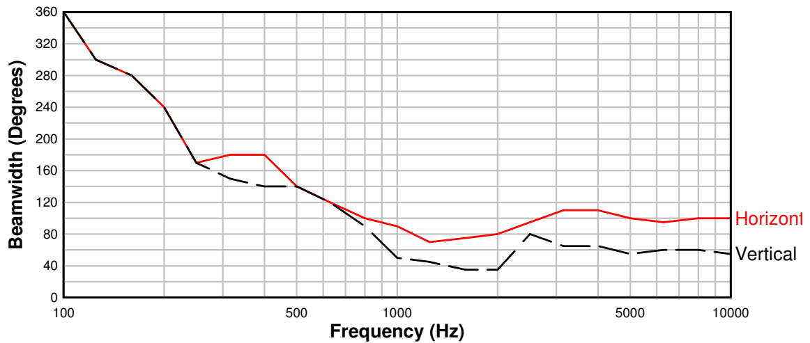
Beamwidth versus Frequency 112IM 105 X 60
